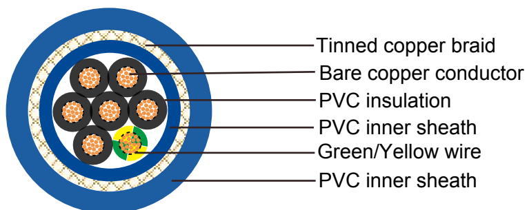
H05VVC4V5-F
